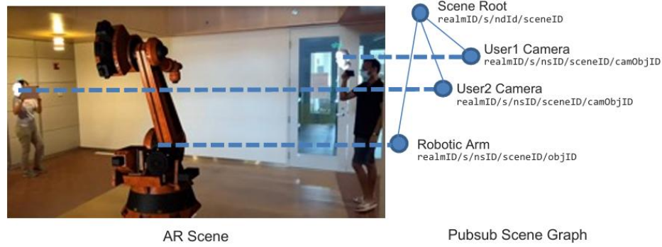
Fig. 3. ARENA Scene The objects in an ARENA Scene are indirectly networked via a PubSub bus where each object is controlled by a topic endpoint. The topic hierarchy is partitioned by Realm (RealmID), owner namespace (nsID), Scenes (sceneID) and objects within the Scene (camObjID or objID)[17].
